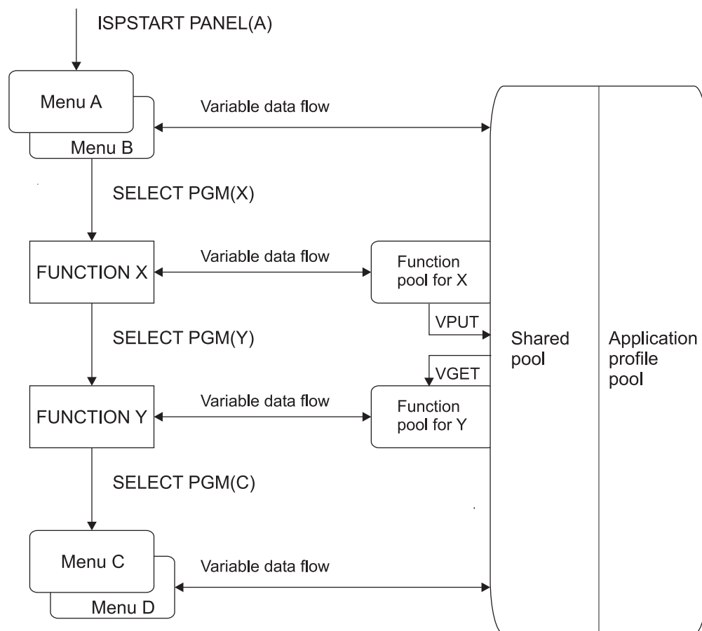
Figure 23. Control and data flow in a dialog
