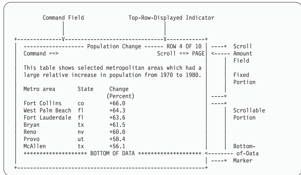
Figure 44. Parts of a TBDISPL display
