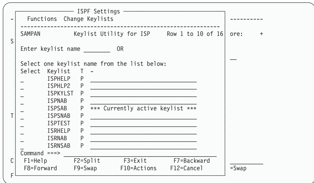
Figure 38. Sample CUA panel (SAMPAN on ISPKLUP)
