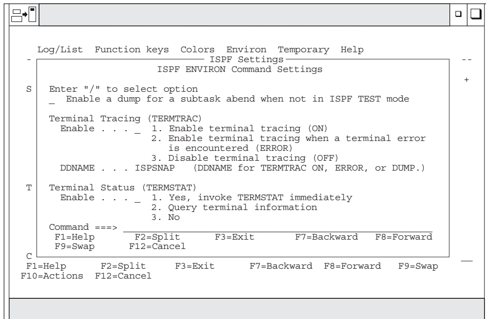
Figure 95. ENVIRON Settings Panel (ISPENVA)
